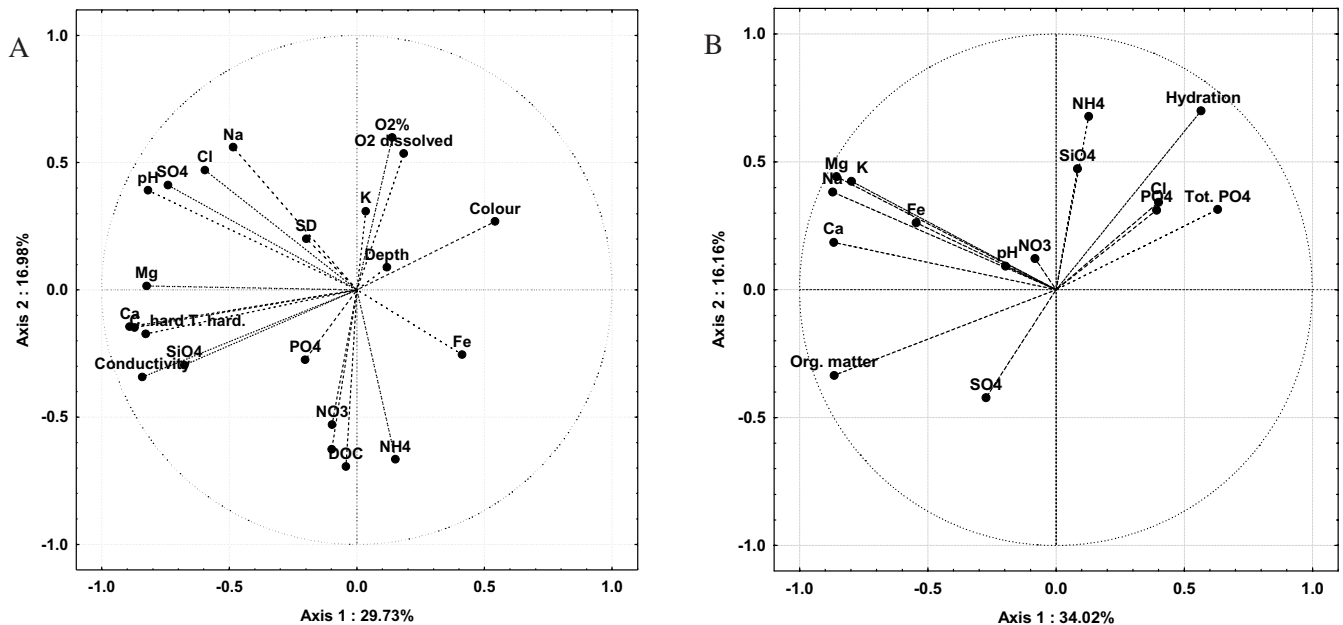
Fig. 1. PCA ordination diagram. The contribution of properties of water (A) and substrate (B) in explanation of the variances observed in associations with dominant nymphaeids
