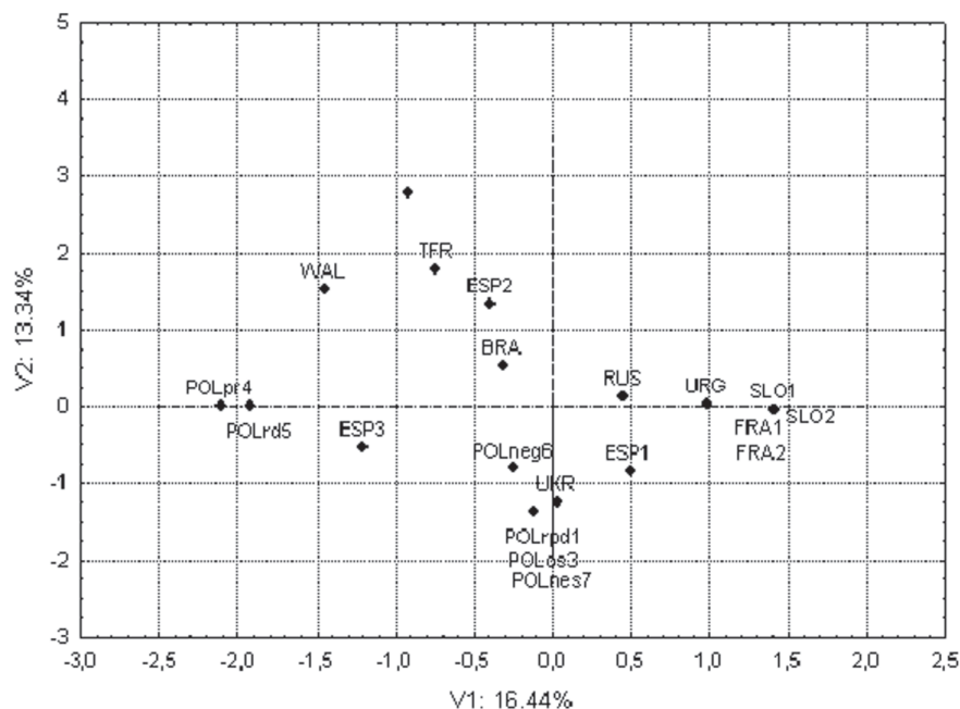
Fig. 2. Scatterplot of 19 A. strigosa ecotypes on principal components based on allele frequencies
