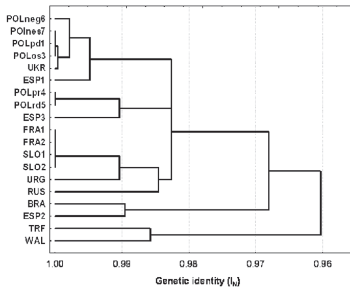
Fig. 1. UPGMA phenogram of 19 A. strigosa ecotypes based on Nei's (1978) genetic identity
