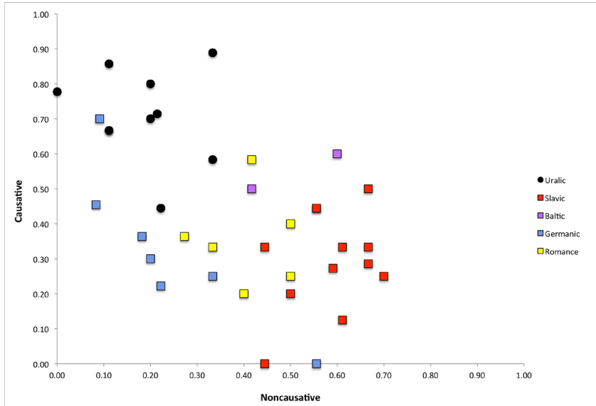
Figure 1. Percent of verb pairs with derived noncausative \times percent with derived causative. Colors identify language families
