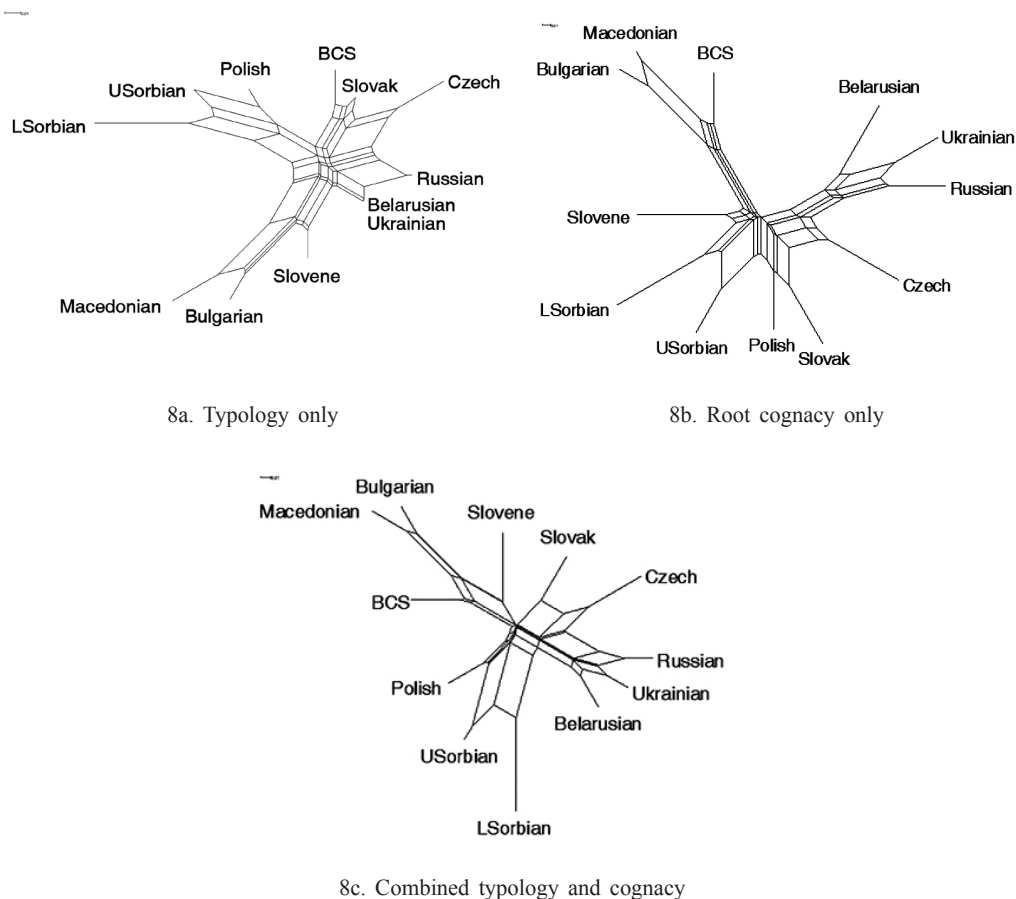
Figure 8. The causative alternation in Slavic: all 18 verb pairs
