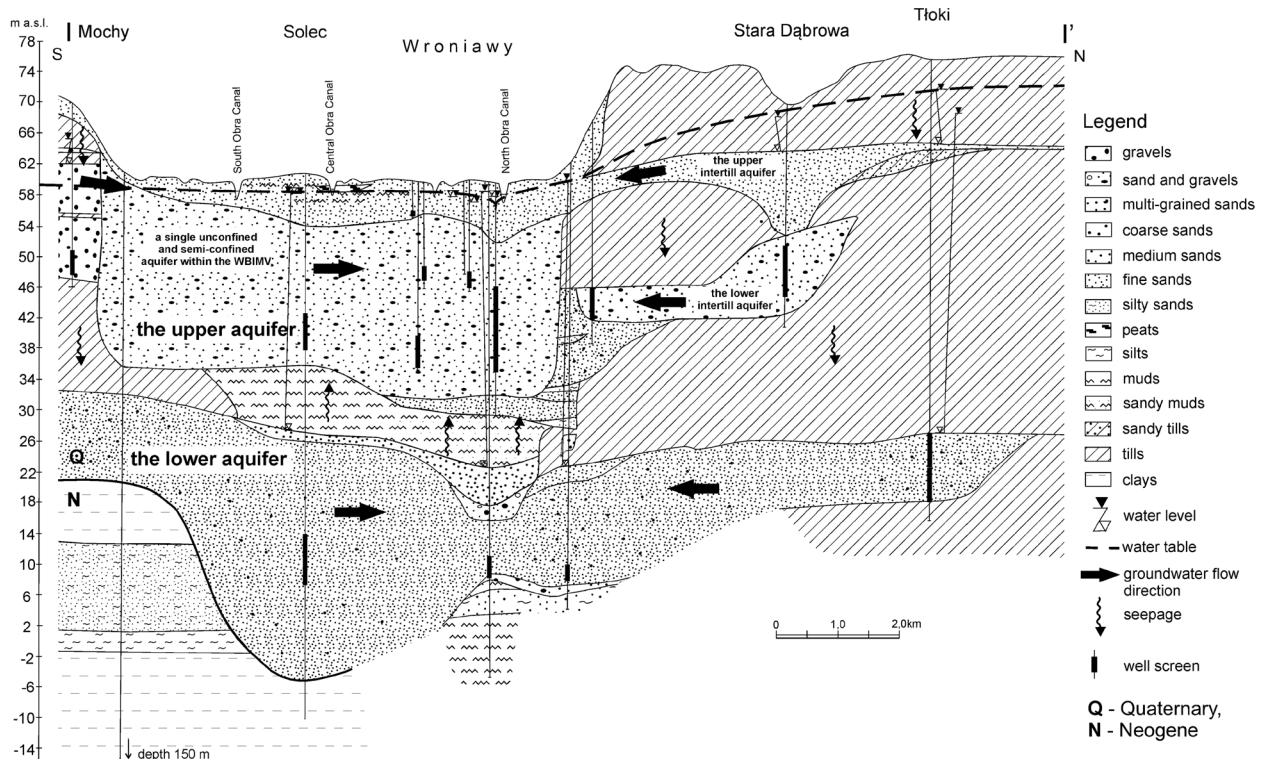
Fig. 2. Hydrogeological cross-section.
