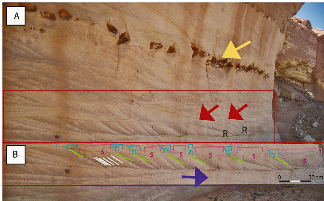
Fig. 9. A – Stacked sandstones strata of FA2. Interspersed mud clasts mark the base of a channel (yellow arrow); B– Closeup view: tidal bundle sequences of neap (n)-spring (s)-neap events (blue and pink intervals) and reactivation surfaces (R – red arrows). Thin white lines trace the internal bundles. Green bounding lines are mud drapes which reflect the cessation of the bedform migration during neap periods. The blue arrow indicates the dominant current direction.
