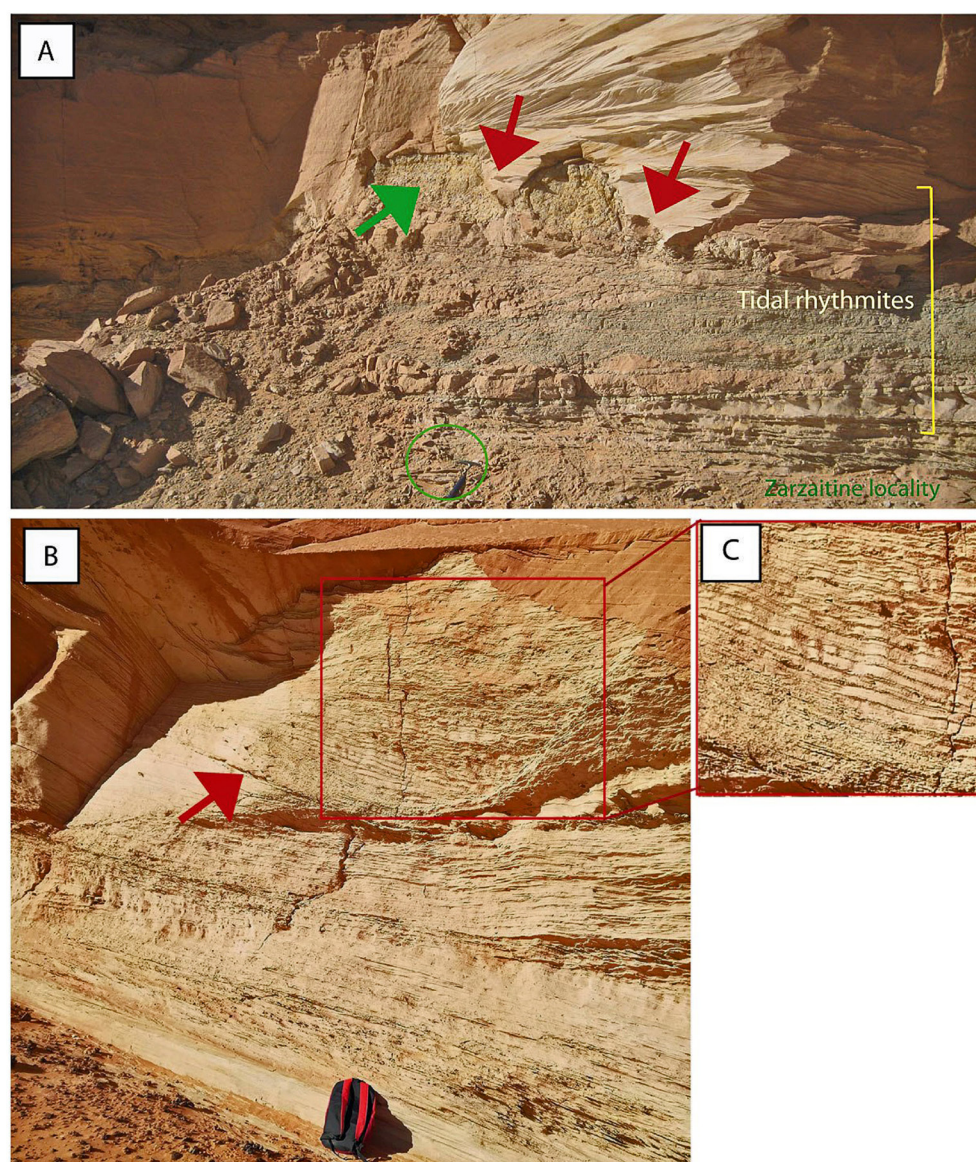
Fig. 8. A – Mud flat deposit (green arrow) and tidal rhythmites (yellow interval) eroded by channels. See basal erosional surface (red arrows). Hammer for scale; B – Tidal rhythmites. See the erosional surface of a channel (arrow); C – Closeup view of tidal rhythmites.
