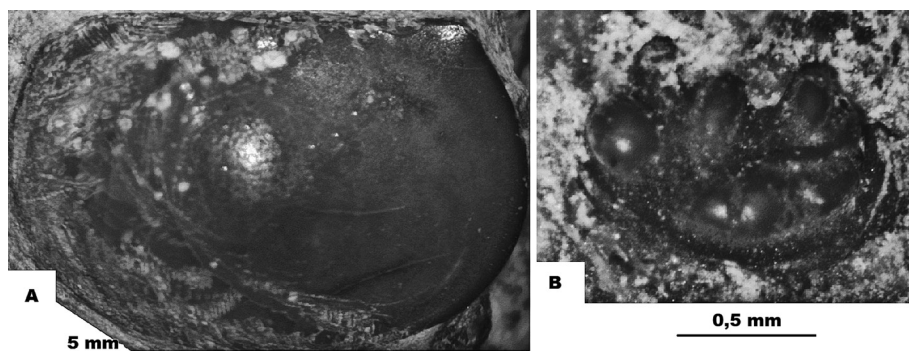
Fig. 7. Ostracods: A - Shell of Leperditia sp., UO-ZP-AK52; B - Shell of a beyrichiid, UO-ZP-AK29.
