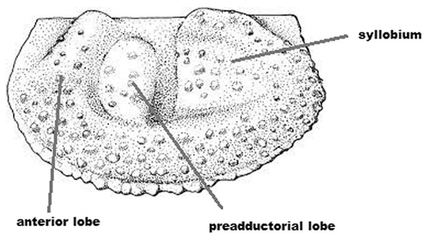
Fig. 5. Beyrichiid shell morphology (based on Siveter, 2022).
