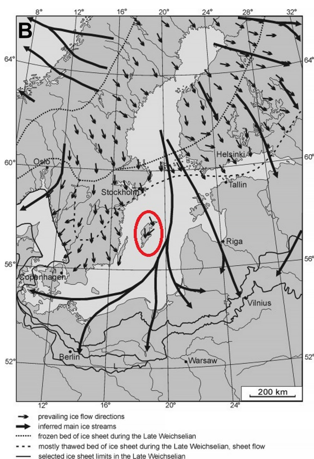
Fig. 8. Places of origin of erratic boulders. A – Map of Baltic Sea Klint and Silurian Klint (based on Soesoo & Mädel, 2007); B – Directions of ice sheet streams during the late Weichselian glaciation (based on Woźniak & Czuba, 2015).
