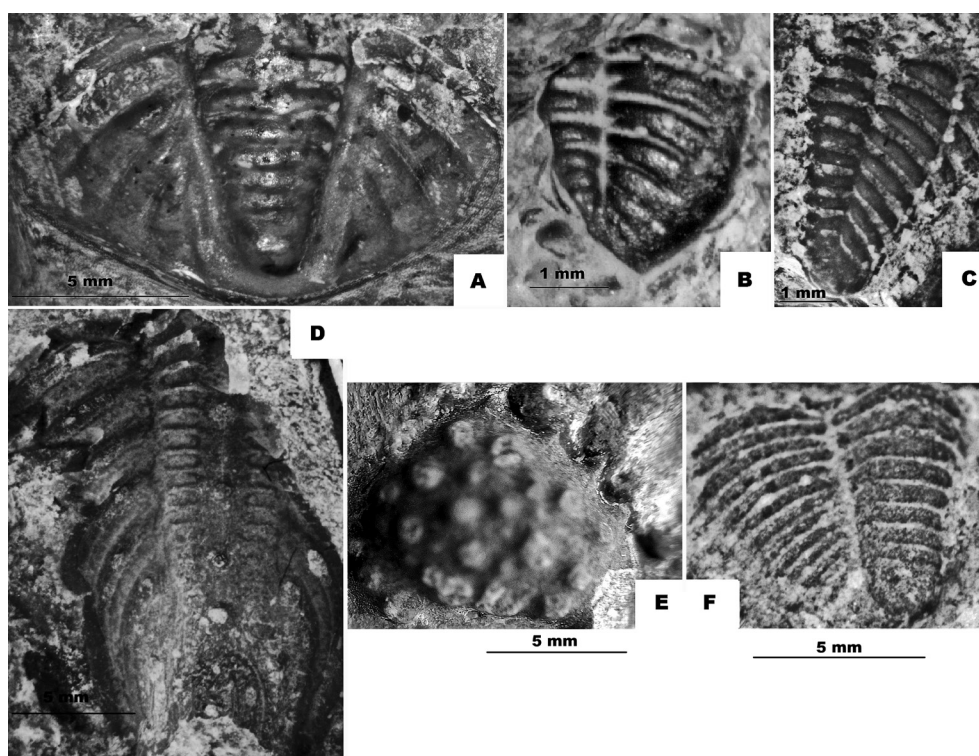
Fig. 6. Trilobites: A – Pygidium of Calymene? sp., UO-ZP-AK05; B – Pygidium of Acaste? sp., UO-ZP-AK06b; C – Pygidium of Chasmopsinae indet., UO-ZP-AK34; D – Pygidium of Encrinurus sp., UO-ZP-AK32b; E – Glabella of Encrinurus sp., UO-ZP-AK32c; F – Pygidium of Proetidae indet., UO-ZP-AK53.
