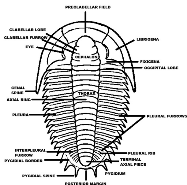
Fig. 4. Trilobite morphology (based on Gon III, 2007).
