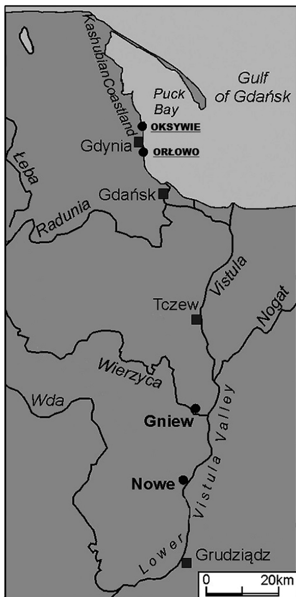
Fig. 1. Location of Orłowo and Oksywie cliffs (based on Woźniak & Czubla, 2016).
