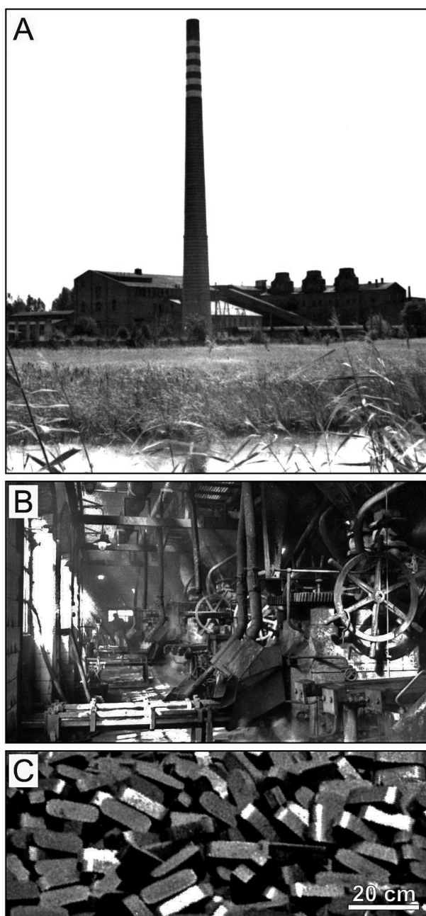
Fig. 2. Briquette factory in Marantów. A – View to the east from the area of the future Gosławice opencast; B – View of the briquette press hall; C – Close-up view of briquettes (photographs from archives of the District Museum in Konin, DMK).
