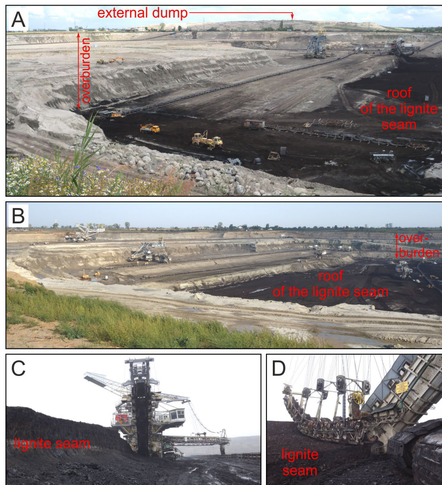
Fig. 9. Tomisławice lignite opencast. A, B – Broad view showing the lignite seam roof and overburden in mid-2024; C, D – Lignite mining by a multi-bucket chain excavator (photographs by M. Widera).
