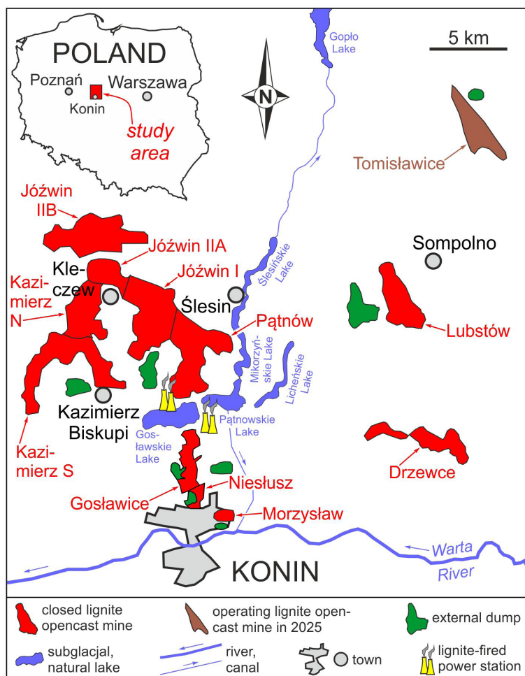
Fig. 1. Location map of opencasts operating in the 80-year history of Konin Lignite Mine (KLM).
