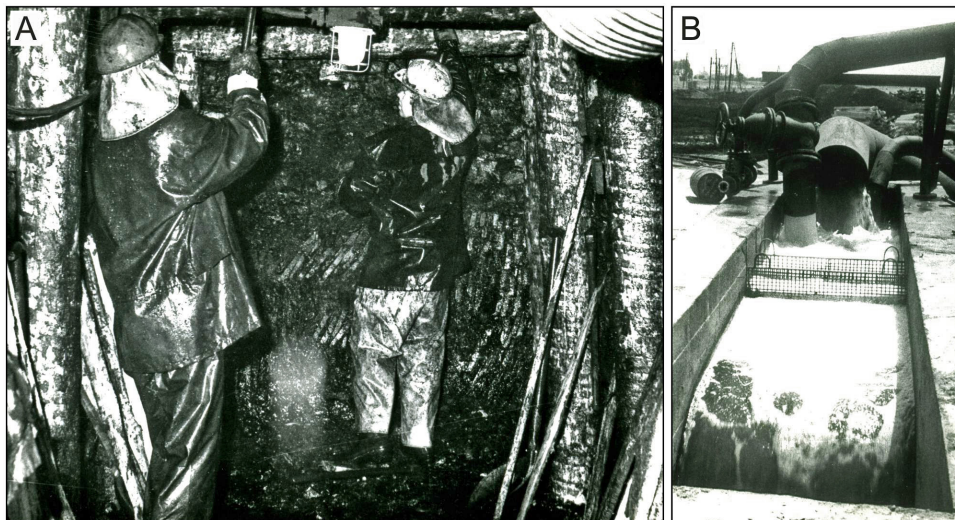
Fig. 8. Underground dewatering system used in the Konin Lignite Mine (KLM) in 1945–1996. A – ‘Seamen from Pątnów’; B – Water from underground dewatering drained into surface channels and rivers (photographs from DMK archives).
