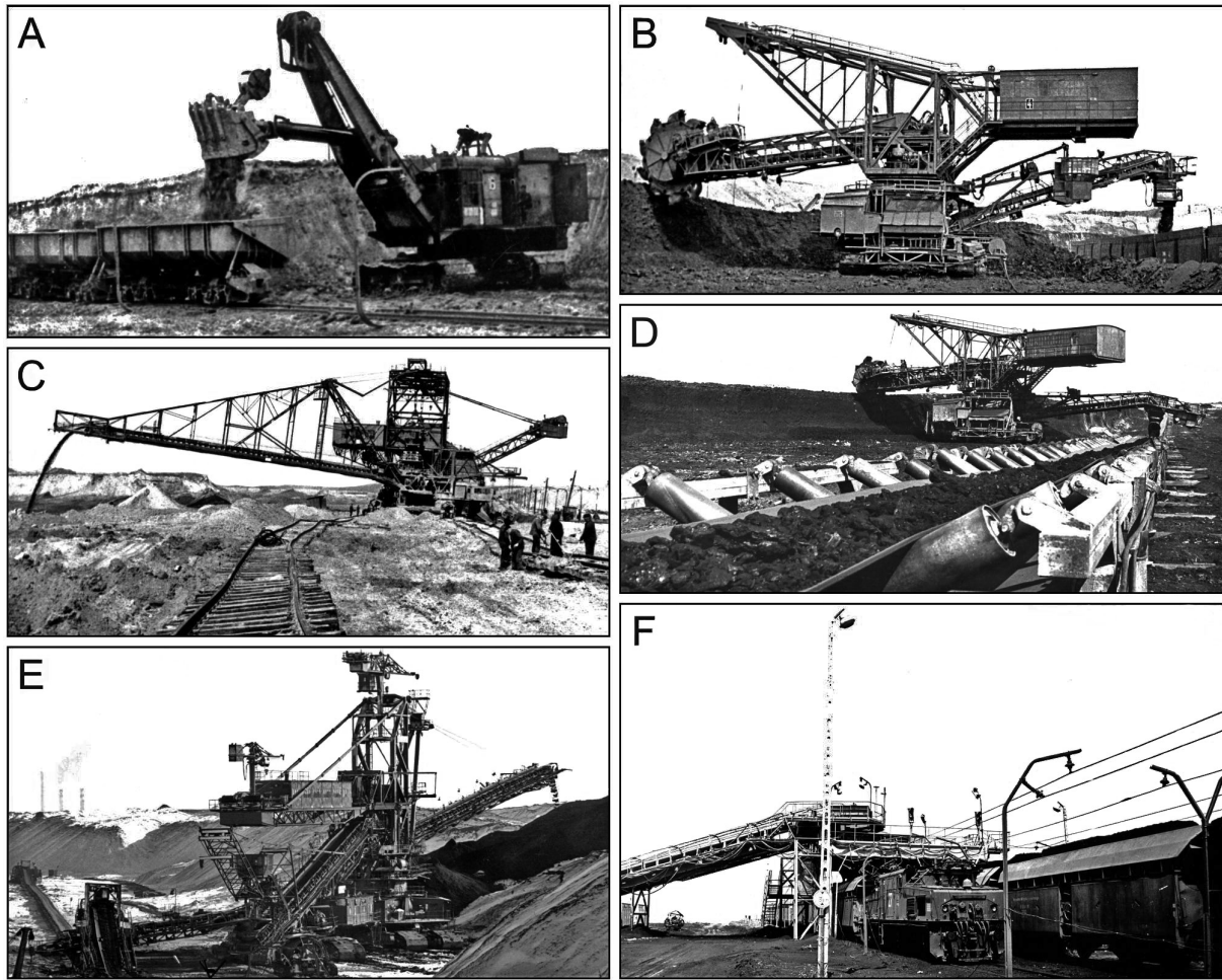
Fig. 7. Technological progress in the Konin Lignite Mine (KLM) during communist times. A-C – From single- to multi-bucket excavators and railway transport; D-F – Predominance of lignite and overburden transport by belt conveyors; note that on the ground surface only lignite is transported by mine railway in Figure 7F (photographs from DMK archives).
