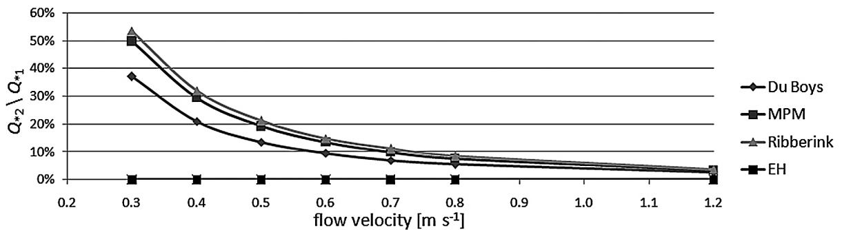
Fig. 11. The Q_{*2} = C_f f(\tau, \tau_{cr}, p) to Q_{*1} = C^* \tau_b^p ratio for models considered as a function of flow velocity.
