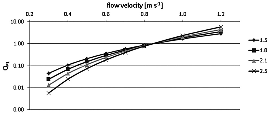
Fig. 10. The dimensionless bed load transport Q_{*1} = C^* \tau_b^p as a function of flow velocity for several values of p power (1.5, 1.8, 2.1, 2.5), C^* = 1 .
