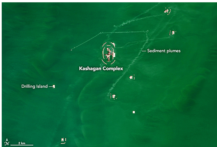
Fig. 1. The Kashagan complex with sediment plumes, indicating water pollution during drilling (NASA aerial photography; http://earthobservatory.nasa.gov/ ).
