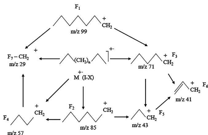
Fig. 3. Fragmentation of n-alkanes (I-X).
