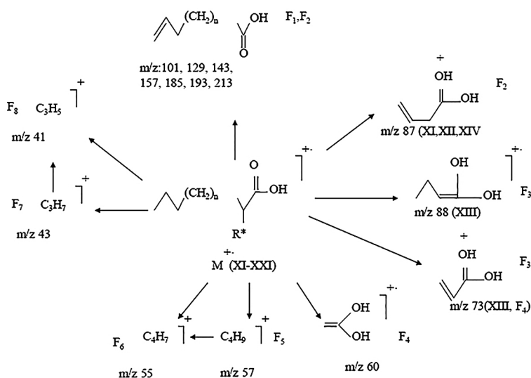
Fig. 4. Fragmentation of aliphatic monocarboxylic acids (XI-XXI).
