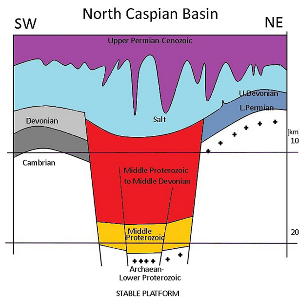
Fig. 5. Cross section through the Caspian Basin, showing the extensive Permian salt diapirs in the stable northern Caspian Basin (after Kroonenberg et al., 2005).
