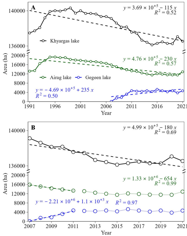
Fig. 6. A – Temporal changes in the water surface area of the Khyargas Lake basin. B – Surface area trends for the water accumulation (2007–2011) and after the accumulation period of Gegeen Lake (2011–2021).
