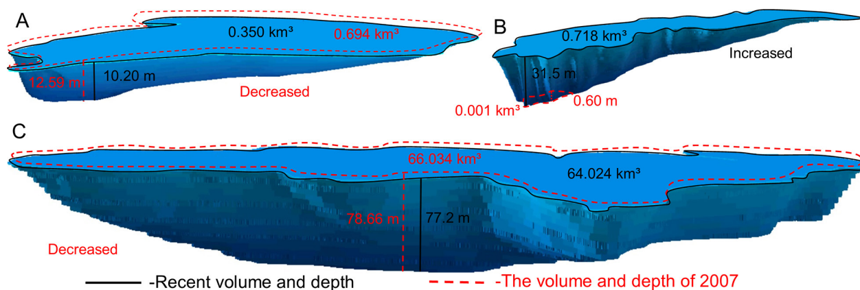
Fig. 9. Three-dimensional model of water volume changes in lakes. Morphometric changes in A – Airag Lake, B – Gegeen Lake and C – Khyargas Lake.
