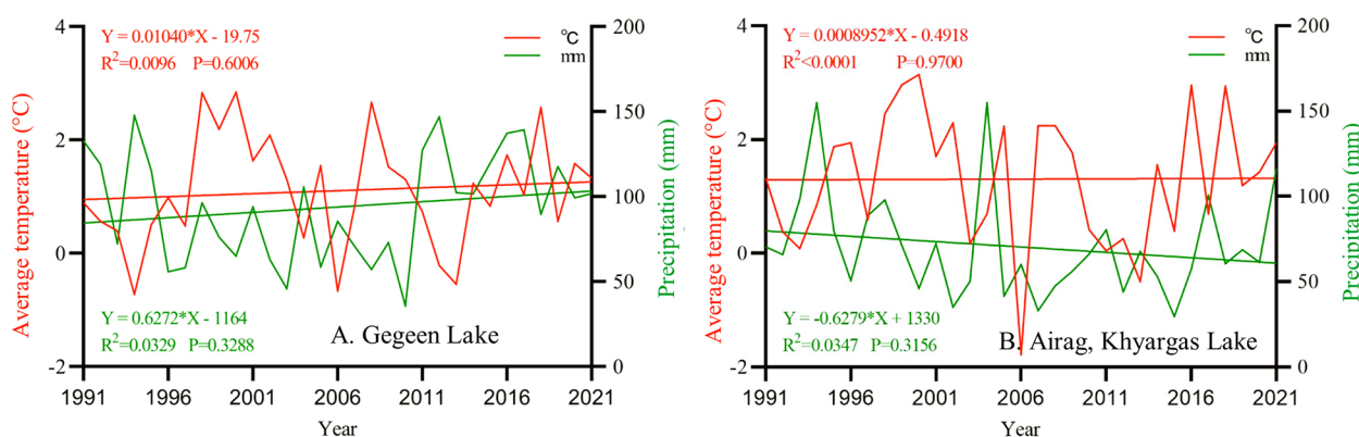
Fig. 11. Climate trends in years 1991–2021.
