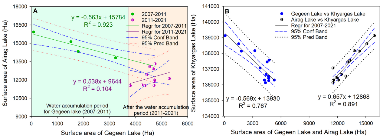
Fig. 7. A – Relationship of surface area changes between the Gegeen and Airag lakes. The light green background represents the water accumulation period for Gegeen Lake, while the light orange background corresponds to the water accumulation period of the lake. B – Relationship of surface area changes for Khyargas Lake with the Gegeen and Airag lakes.
