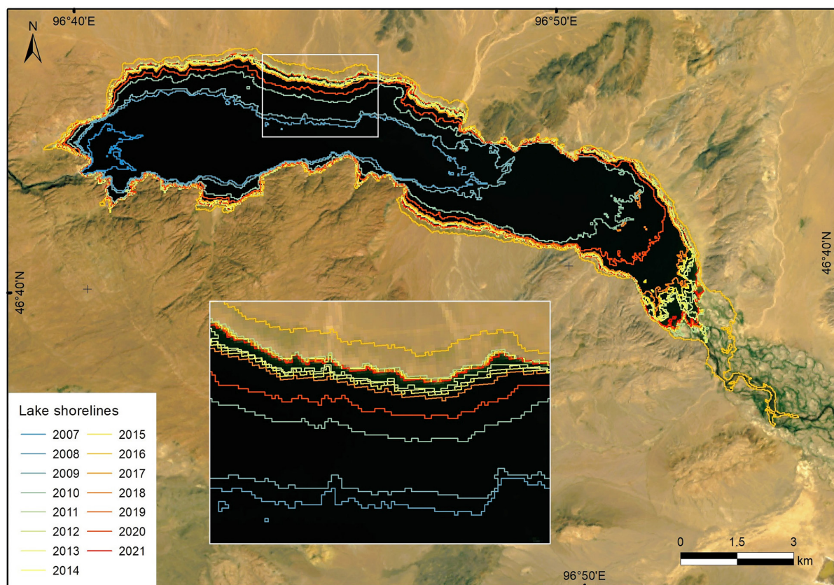
Fig. 4. Morphological changes in the area of Gegeen Lake (2007–2021).
