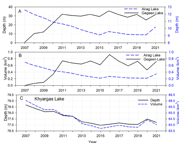
Fig. 8. Variations in morphometric changes in the lakes. A – Depth change; B – volume change of the Airag and Gegeen lakes and C – depth and volume changes of Khyargas Lake.
