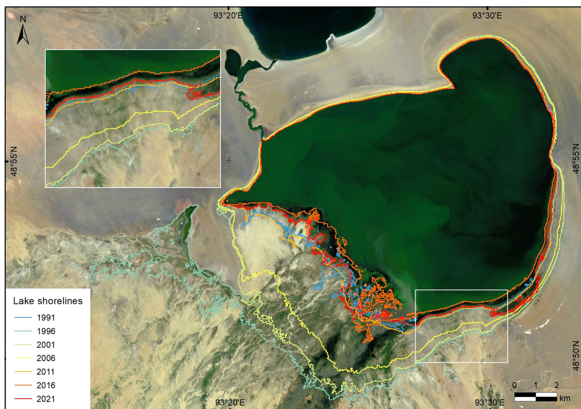
Fig. 3. Morphological changes in the area of Airag Lake (1991–2021).
