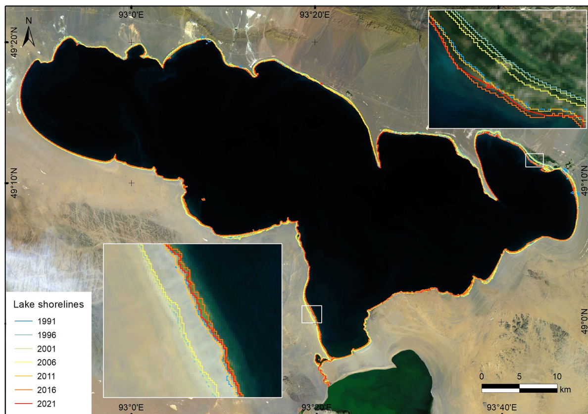
Fig. 5. Morphological changes in the area of Khyargas Lake (1991–2021).
