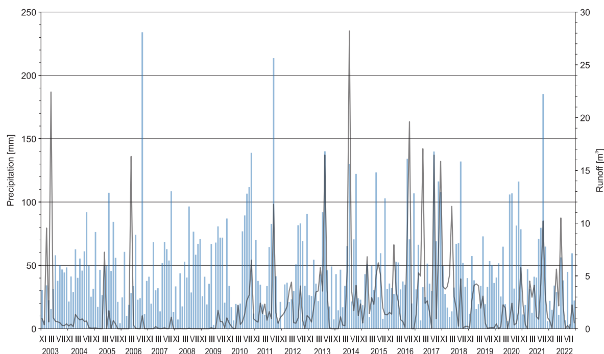
Fig. 5. Monthly precipitation total sum and runoff between 2003 and 2022 in the studied gully catchment.
