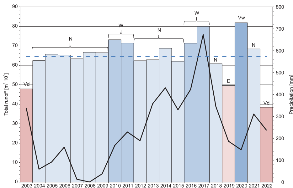
Fig. 3. Distribution of annual sums of precipitation and annual volumes of water runoff from the gully catchment for the years 2003–2022; precipitation classification according to Kaczorowska (1962): Vd – extremely dry year, D – dry year, N – average, W – wet, Vw – extremely wet and blue dotted line means the average precipitation for total period.
