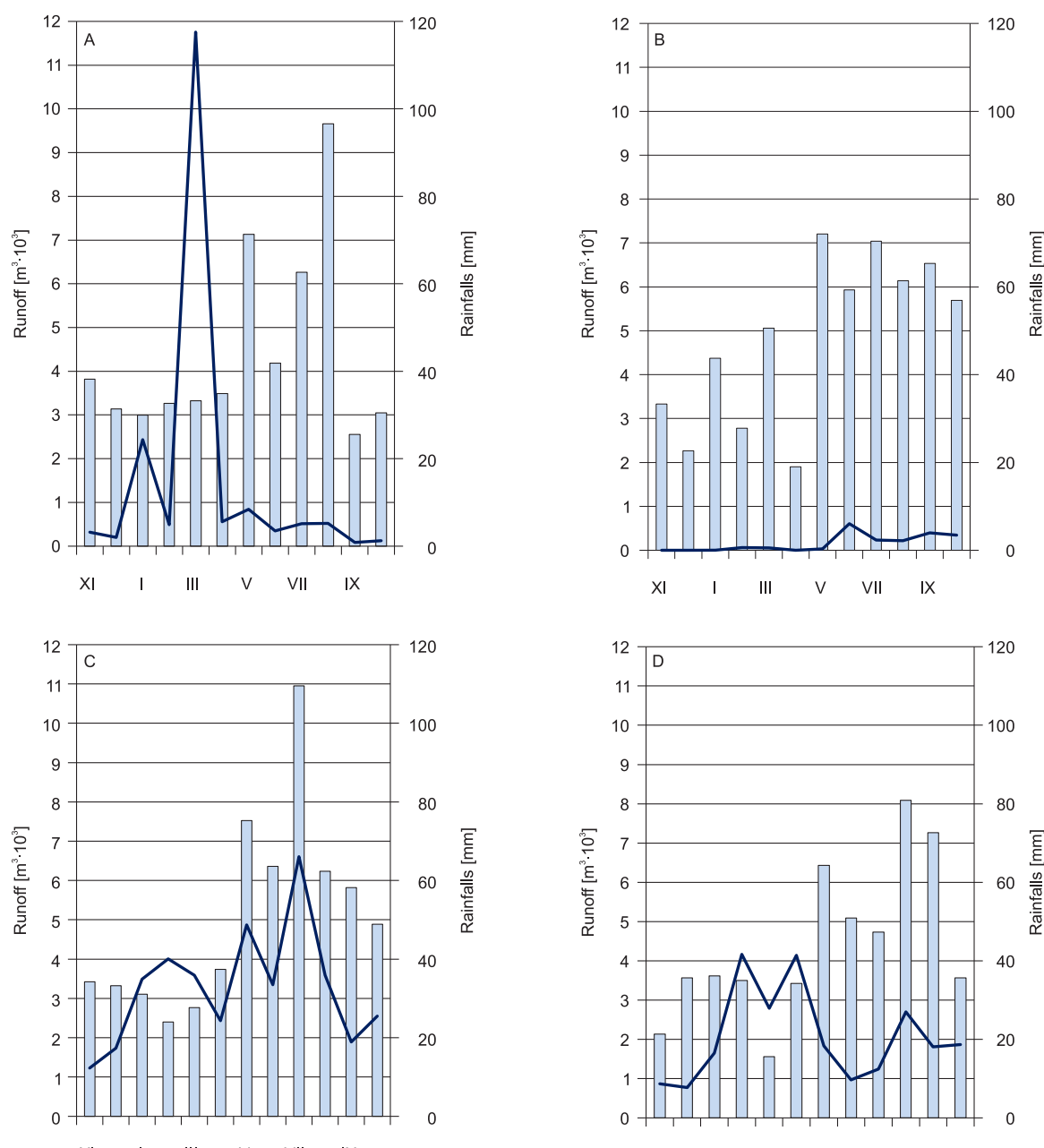
Fig. 7. Average monthly precipitation total sums and runoff in the gully catchment: A – nival period 2003–2006, B – steady period 2007–2009, C – pluvial period 2010–2018, D – variable period 2019–2022.
