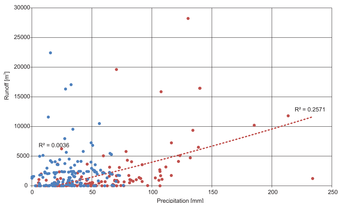
Fig. 9. Response of a loess gully catchment water runoff to a downpours series depending on the preceding conditions: A – during the dry period, B – during the wet period.
