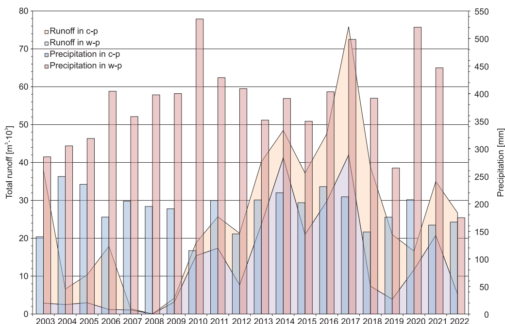
Fig. 4. Distribution of half-year precipitation and water runoff from studied gully catchment in Kolonia Celejów in 2003–2022; c-p – cold half-year, w-p – warm half-year.
