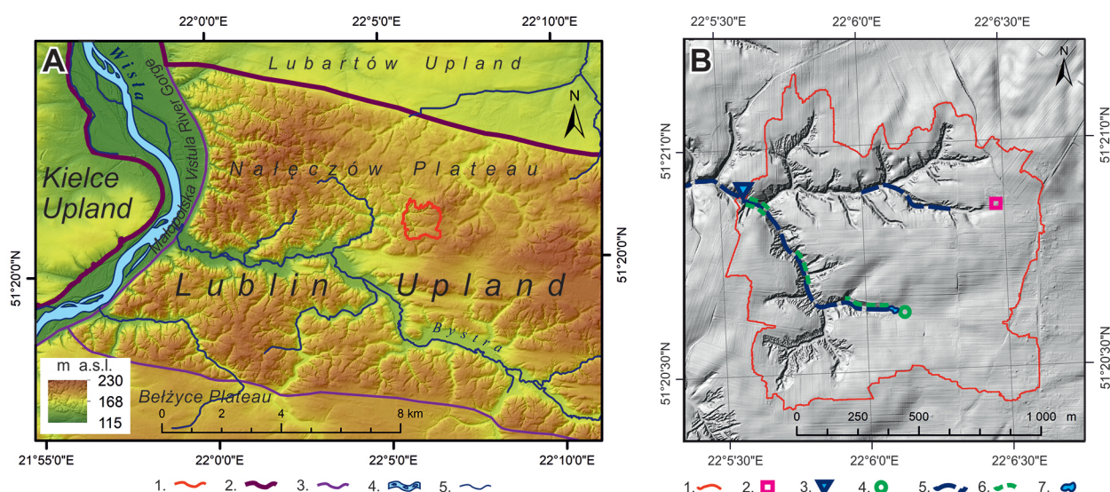
Fig. 1. A – Localisation of the study area on the DEM background: 1 – Kolonia Celejów catchment, 2 – macroregions border, 3 – mesoregions border, 4 – the Vistula channel, 5 – stream channel; B – Relief and hydrological conditions of the studied catchment in Kolonia Celejów (Hillshade Relief Model – DEM: https://mapy.geoportal.gov.pl ): 1 – catchment border, 2 – rainfall station, 3 – hydrological station, 4 – spring, 5 – periodical stream, 6 – seeps and exudates, 7 – pond.
