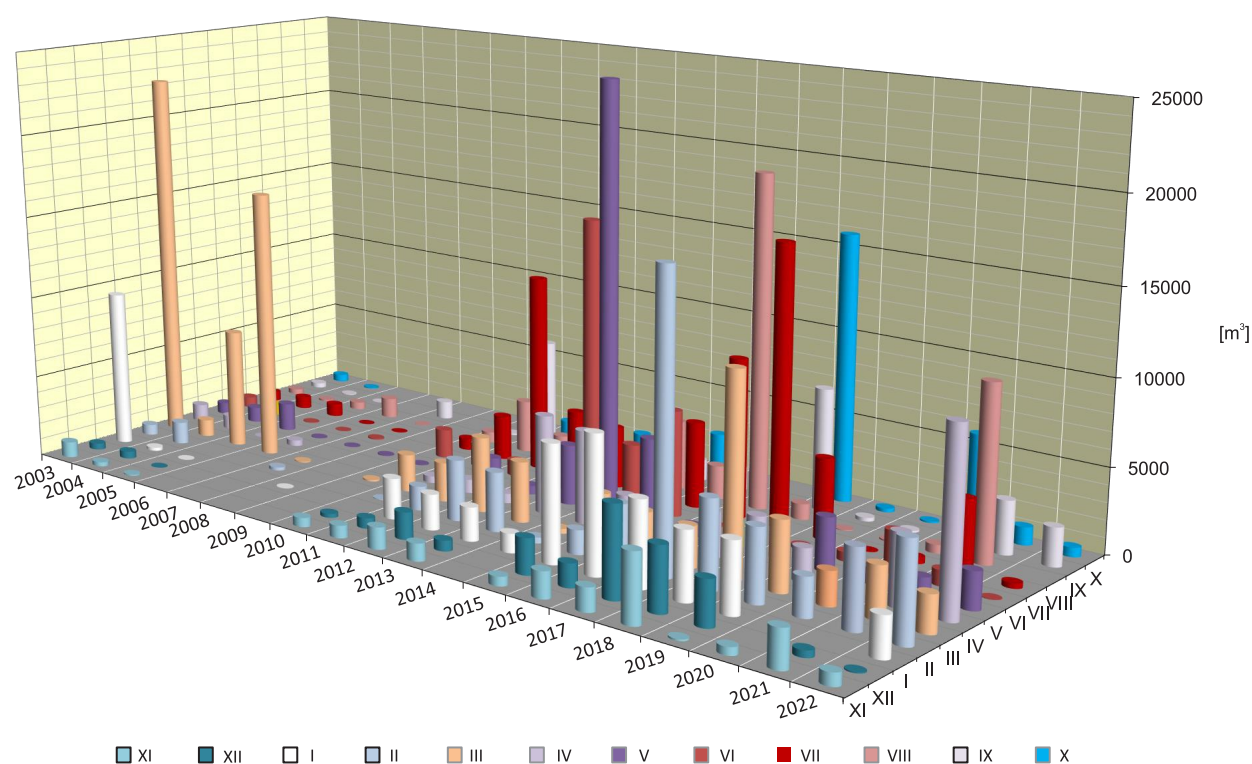
Fig. 6. Monthly water runoff sums distribution from the loess gully catchment Kolonia Celejów in the 20-year period 2003–2022.
