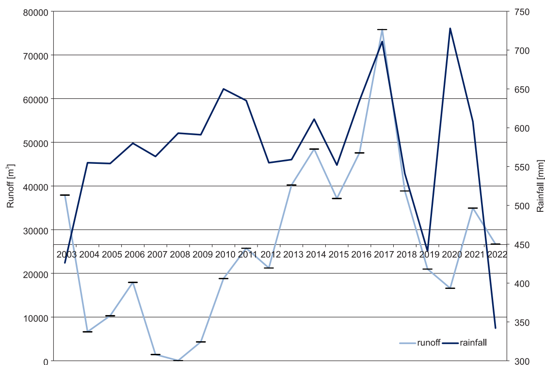
Fig. 8. Multi-year distribution of the precipitation total sums and annual runoff between 2003 and 2022 from the gully catchment. Position of X axis determines the average annual water runoff from the catchment.
