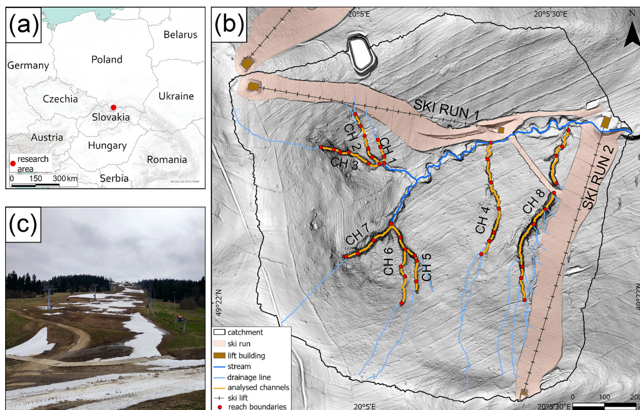
Fig. 1. Location of the study area: A – a regional overview, B – a hillshaded relief of the catchment with analysed channels. Channels are signed with CH and followed numbers. Important drainage lines and ski infrastructure are marked, and C – a photograph of the catchment with ski run 2 (photo: D. Piątek).
