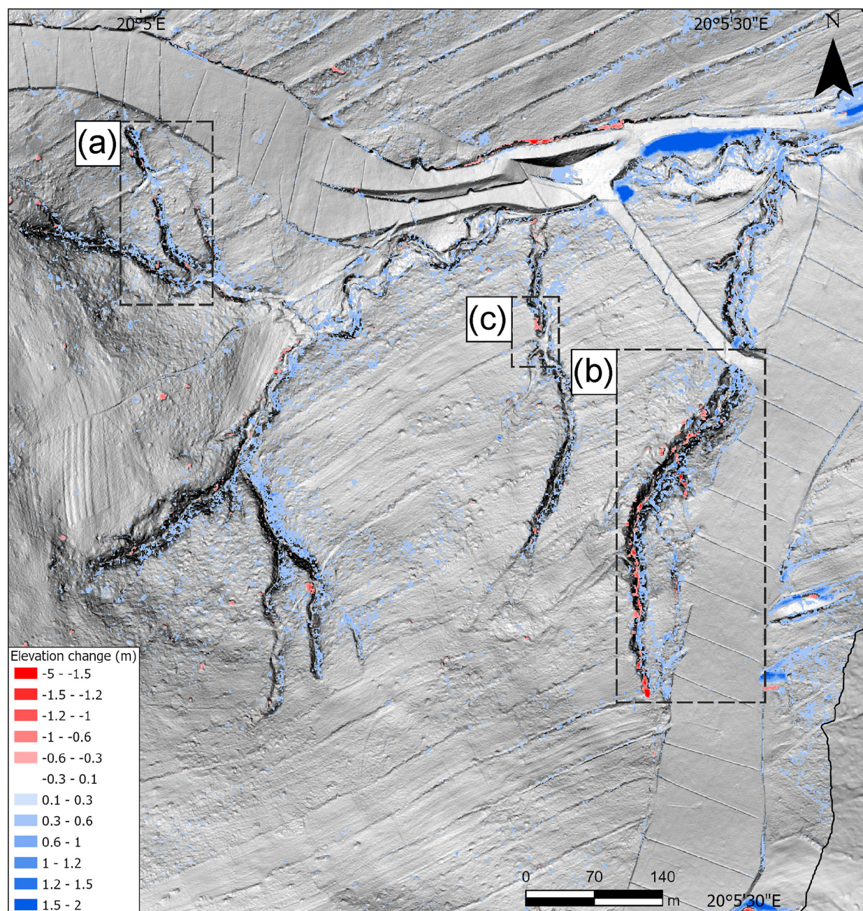
Fig. 7. Elevation changes in analysed channels in the period 2016–2023, in rectangle areas presented in Figure 8.
