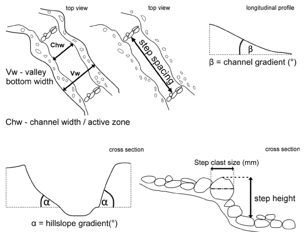
Fig. 2. Schematic diagram of selected measurements, black arrows and Greek letters show the way of measurement.
