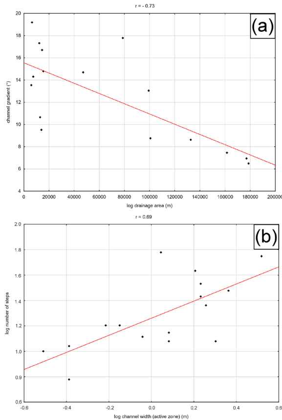
Fig. 6. Distinctive correlations in the group of channels affected by ski runs (reach averaged data), A – drainage area versus channel gradient; B – channel width versus number of steps.
