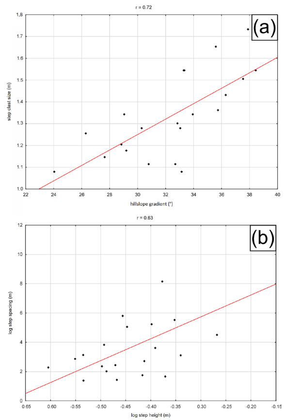
Fig. 5. Distinctive correlations in the group of channels without impact of ski runs (reach averaged data), A – hillslope gradient versus step clast size; B – step height versus step spacing.
