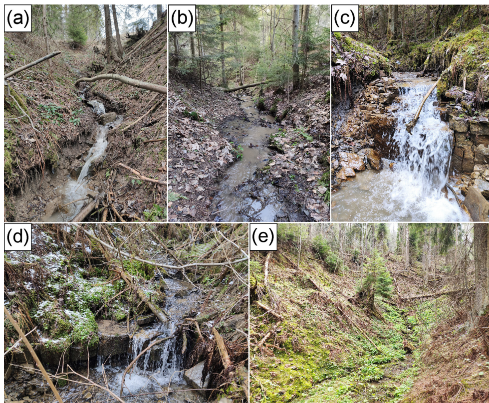
Fig. 3. Photographs of characteristic parts of analysed channels: A – a part of Channel 2 with traces of lateral and deep erosion, B – a part of Channel 4 with a relatively high gradient, C – a part of Channel 8 with a 0.6-m-high step below the rockfloor, D – a step with typical height for catchment, Channel 3, E – part of Channel 7, fulfilled with material from a small landslide visible in the left corner (photos: A. Gołąb and D. Piątek).
