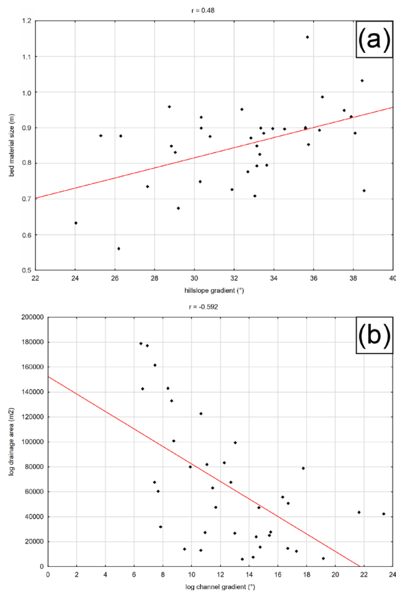
Fig. 4. Distinctive correlations in the group of all analysed channels (reach averaged data), A – hillslope gradient versus bed material size; B – channel gradient versus drainage area.
