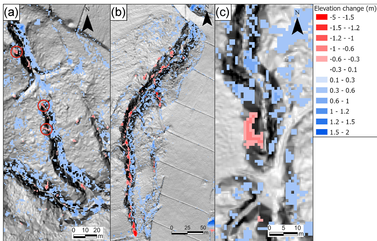
Fig. 8. Close up on areas with elevation changes marked with rectangles on Figure 7; A – close up on Channel 2, in red rings marked results of headward erosion; B – close up on Channel 8 with zones with erosion and deposition; and C – close up on a small landslide on hillslopes of Channel 4.
