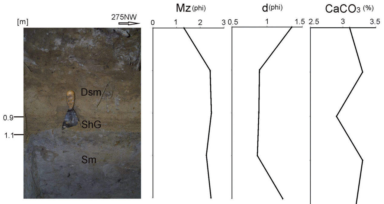
Fig. 2. Geological profile of the proximal part of alluvial cone with its grain-size distribution values and CaCO 3 content.
