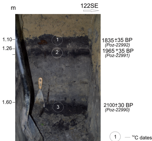
Fig. 3. Geological profile of the distal part of alluvial cone.
