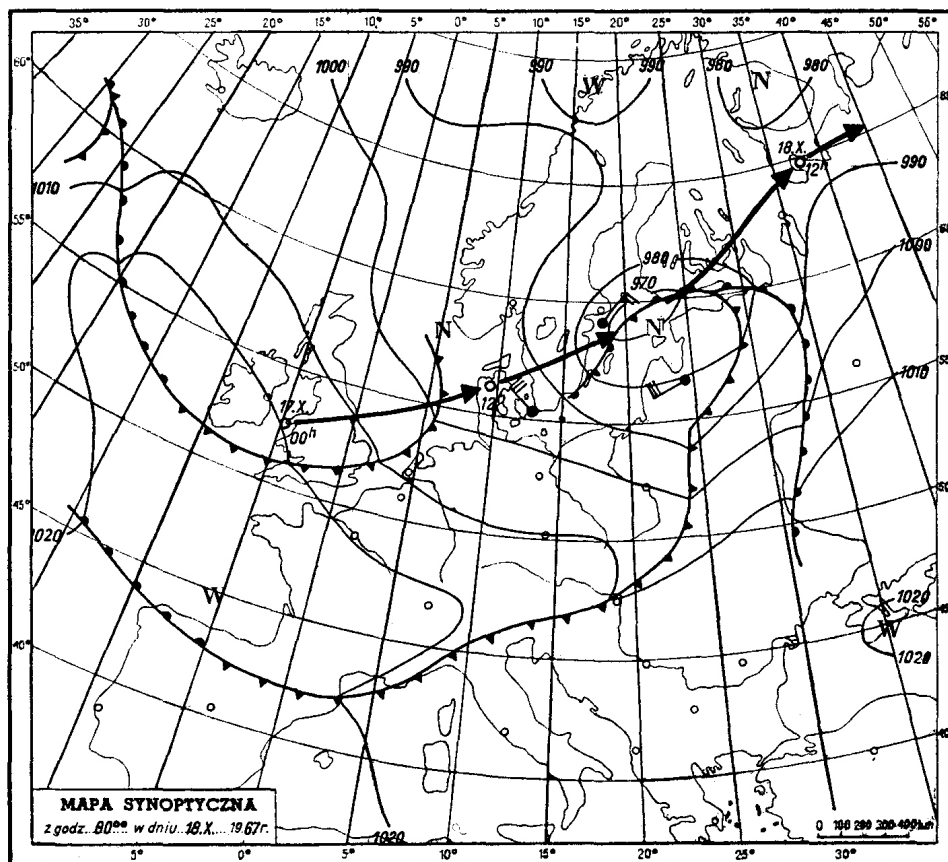
Fig. 2. Synoptic chart of the 18 October 1967 event
