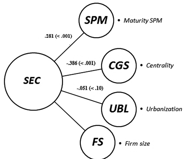
Figure 11. A path model for high-tech spaces and efficient firms.
