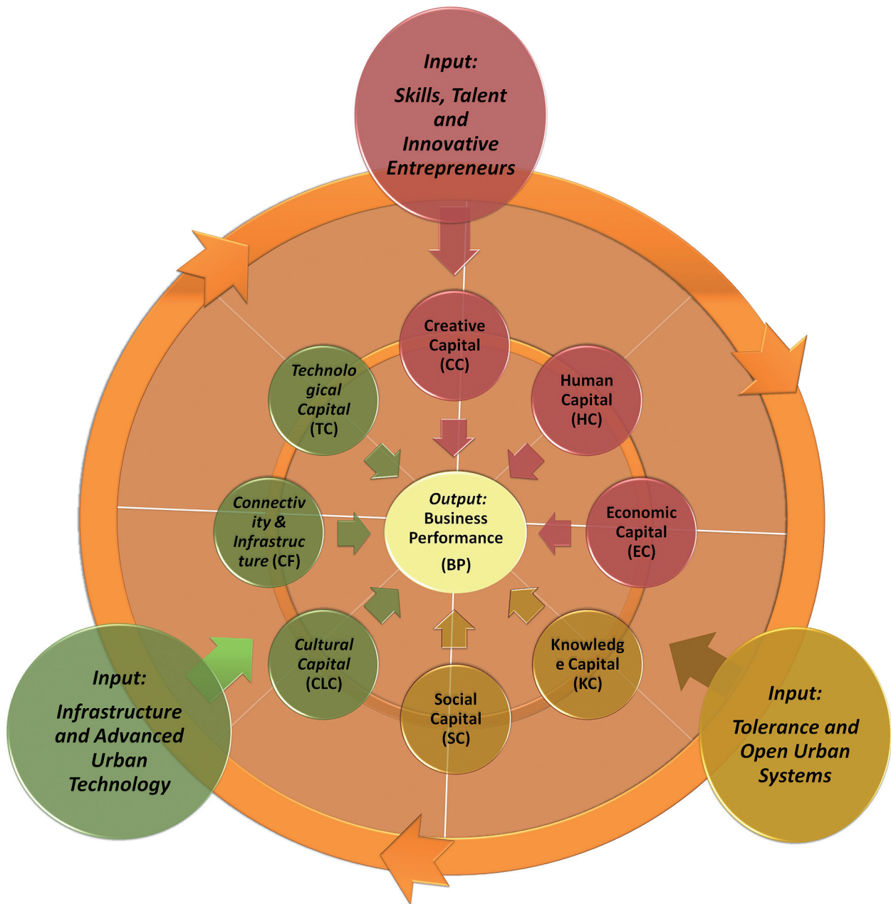
Fig. 9. Architecture of the 'Flying Disc' model of firms' business performance in geographical space.
